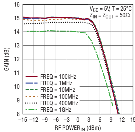
Gain vs RF Power In Over Frequency
