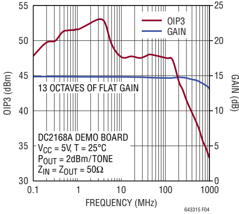
Figure 4. DC2168A Gain and OIP3 vs Frequency
