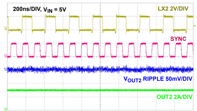
FIGURE 26. STEADY STATE OPERATION CHANNEL 2 3A LOAD WITH F_{SW} = 4\text{MHz}
