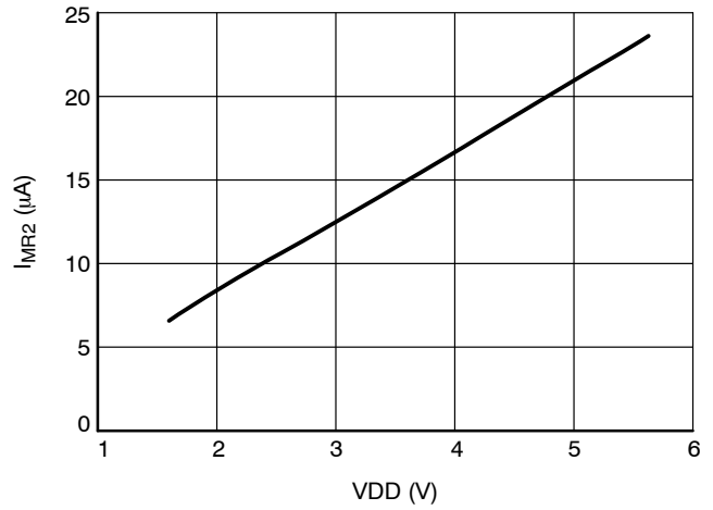
Figure 8. I_{MR2} @ MR2 = 0
