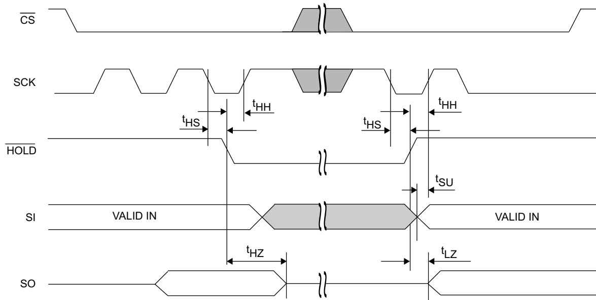
Figure 17. \overline{HOLD} Timing
