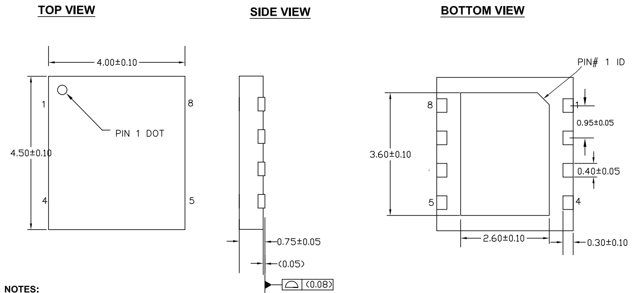
Figure 19. 8-pin DFN ( 4.0 \times 4.5 \times 0.8 mm) Package Outline, 001-85260
