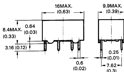
G5A-237P, G5A-237PH, G5A-237P-FC
