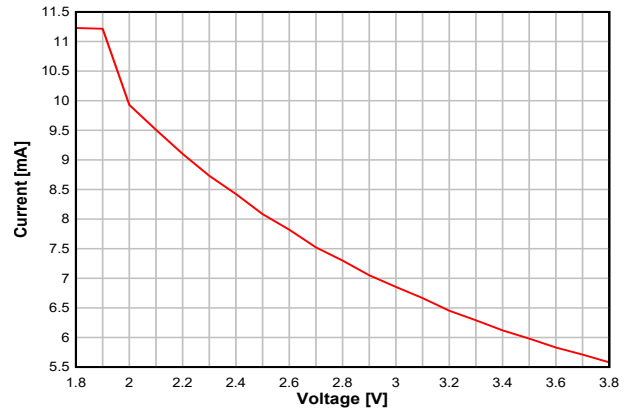
Figure 7-7. RX Current vs. Supply Voltage (VDD5) (BLE 1Mbps, 2.44GHz)
