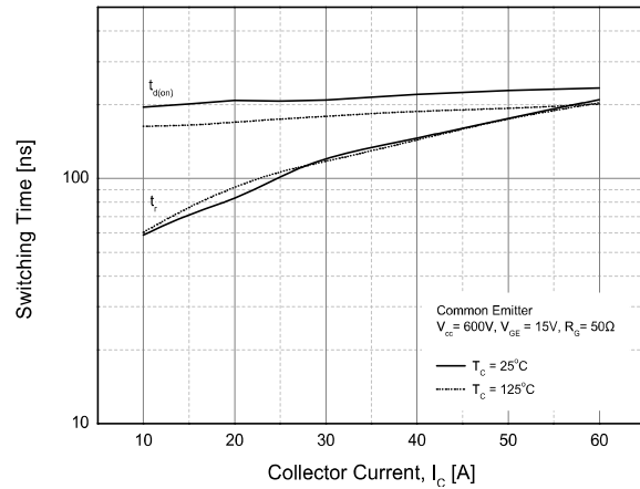
Fig. 10 Turn on time vs. collector current
