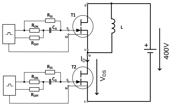
Figure 23 Switching times with inductive load
