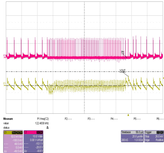
CH1: Vout (50mV/div); 20uS/div CH2: PHASE (10V/div) Figure 11: FCCM/CCM transition from 0.5A to 5A at 12.6V IN : 30mV overshoot, 15mV undershoot
