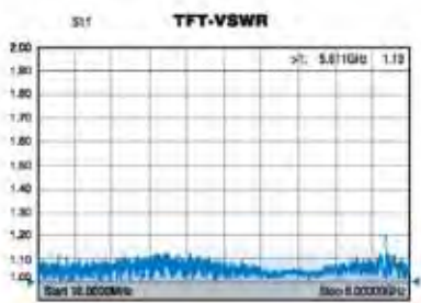
Typical VSWR
