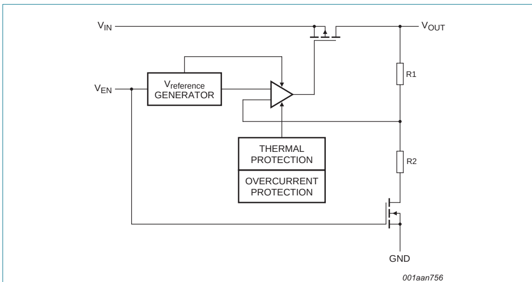
Fig 3. Block diagram of LD6836x/xxH
