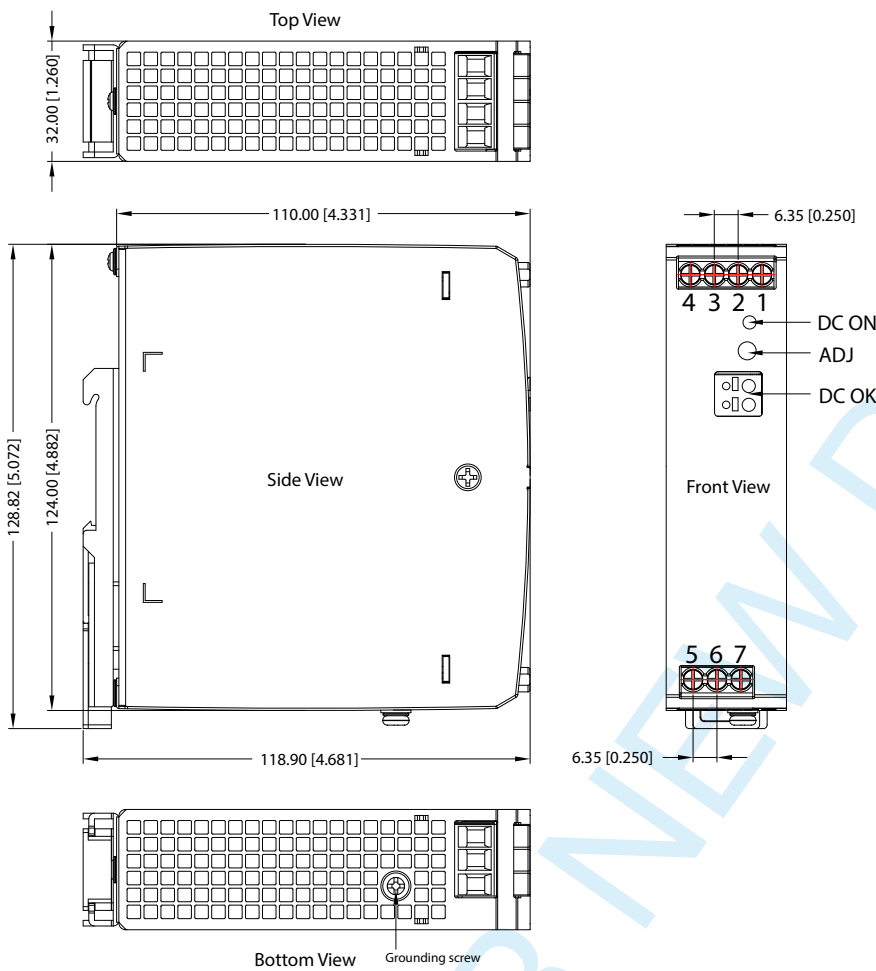
Figure 5. Mechanical Drawing
