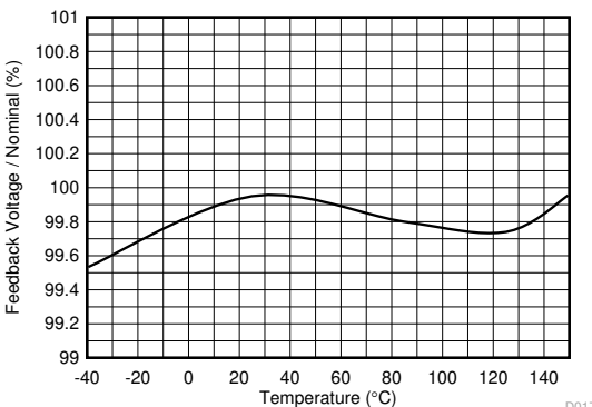
Figure 7-5. Normalized V_{FB} vs Temperature
