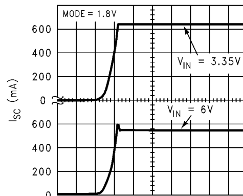
TIME (500 μs/DIV)
