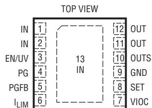
DD PACKAGE 12-LEAD (3mm × 3mm) PLASTIC DFN T JMAX = 150°C, θ JA = 34°C/W, θ JC = 5.5°C/W EXPOSED PAD (PIN 13) IS IN, MUST BE SOLDERED TO PCB
