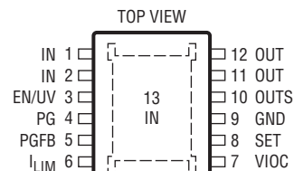
MSE PACKAGE 12-LEAD PLASTIC MSOP T JMAX = 150°C, θ JA = 33°C/W, θ JC = 8°C/W EXPOSED PAD (PIN 13) IS IN, MUST BE SOLDERED TO PCB
