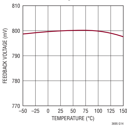
Feedback Voltage
