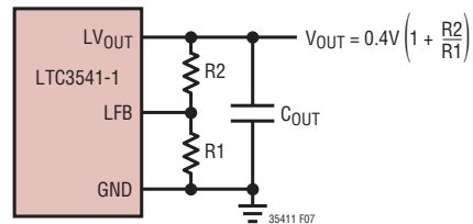
Figure 7. Programming the LTC3541-1
