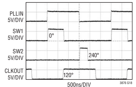
Phase Relationship: PHASMD = INTVCC (Forced Continuous Mode)
