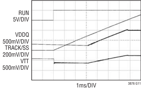
Soft Start-Up Into Prebiased Output
