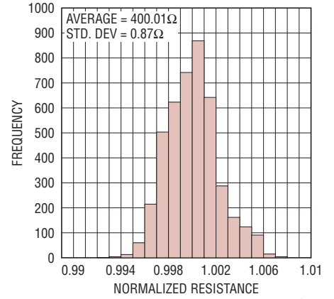
Normalized Feedback 400Ω Resistor Trim
