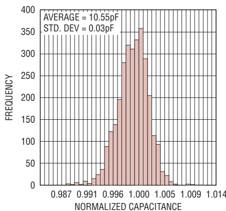
Normalized 10.55pF Capacitor Trim
