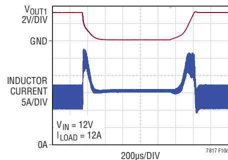
Short-Circuit Response
