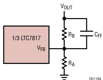
Figure 4. Setting Buck Output Voltage
