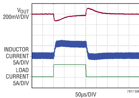
Load Step (Buck) Forced Continuous Mode
