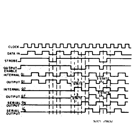
Fig. 3 - Timing diagram.
