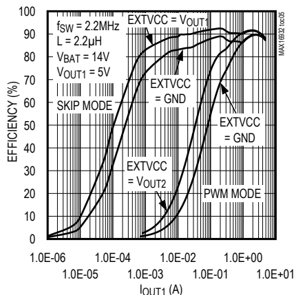
BUCK1 EFFICIENCY
