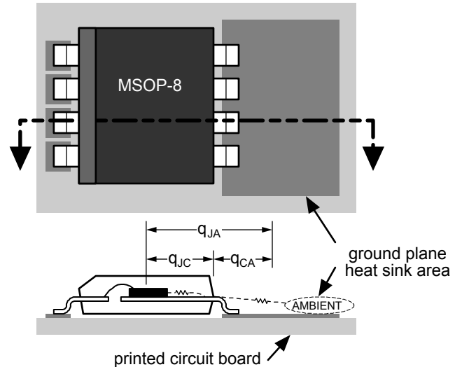
Figure 1. Thermal Resistance
