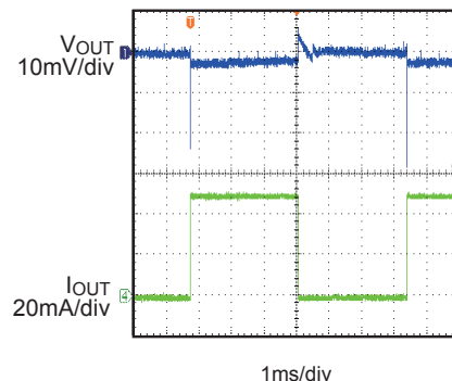
Load Transient Response I_{OUT}=0 to 50mA
