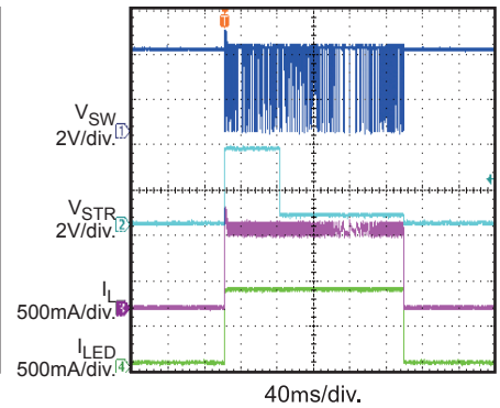
Flash Mode with Edge Trigger Way
