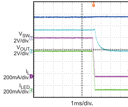
Torch/Assist Mode LED_EN Bit Disable
