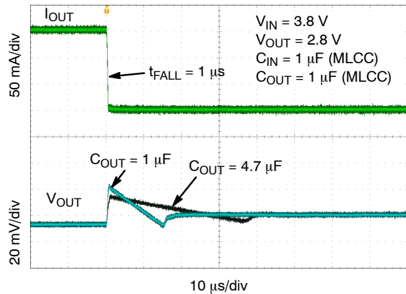
Figure 37. Load Transient Response – Falling Edge, V_{OUT} = 2.8\text{ V} , I_{OUT} = 1\text{ mA} to 150\text{ mA} , C_{OUT} = 1\text{ }\mu\text{F} , 4.7\text{ }\mu\text{F}
