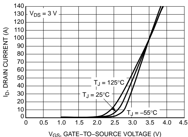
Figure 15. Transfer Characteristics
