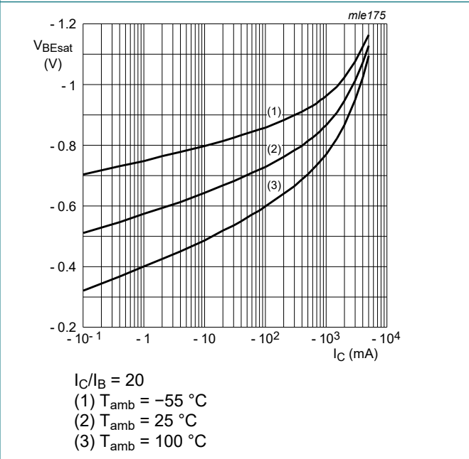
Fig. 12. Base-emitter saturation voltage as a function of collector current; typical values
