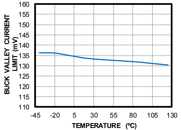
Buck Valley Current Limit vs. Temperature, I LIM = 111b
