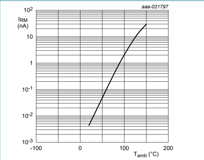
Fig. 7. Relative variation of reverse leakage current as a function of ambient temperature; typical values VRWM = 15 V
