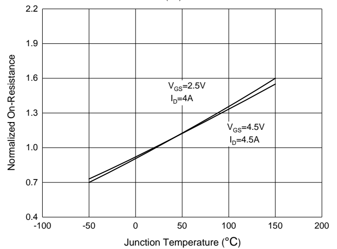
Fig. 4 - R_{DS(ON)} —Temperature
