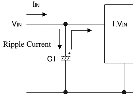
Fig.8 Current Flow of C1
