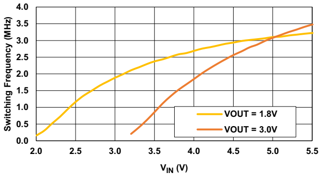
Figure 11. Switching Frequency vs Input Voltage: I OUT = 600mA
