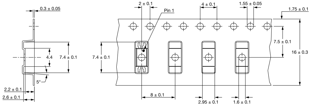
Fig. 17 - Tape and Reel Shipping Medium
