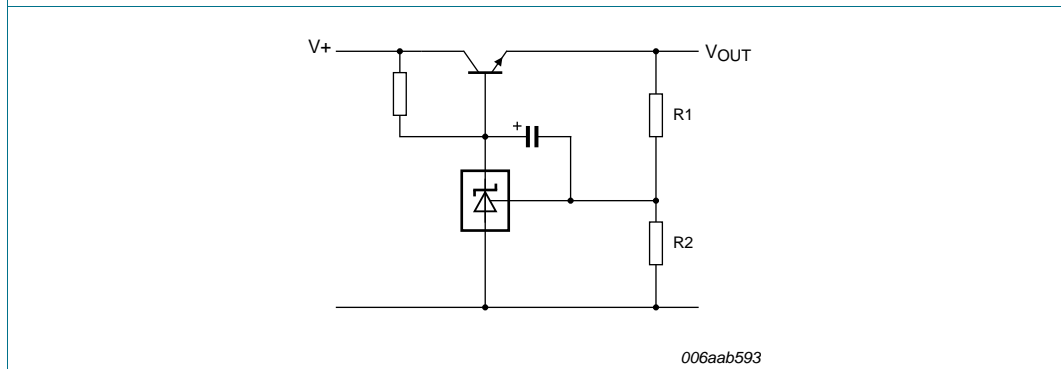
Fig 24. Shunt regulator
