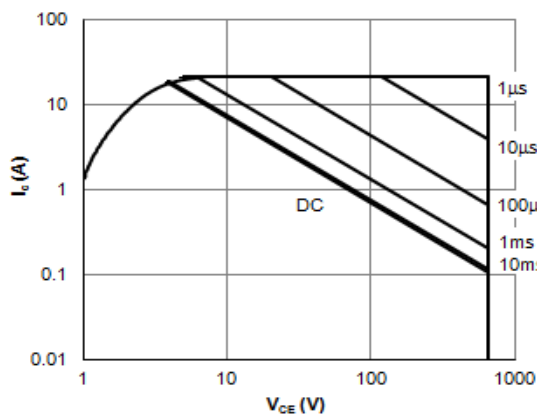
Figure 9: Forward Bias Safe Operating Area ( T_c=25^\circ\text{C}, V_{CE}=15\text{V} )
