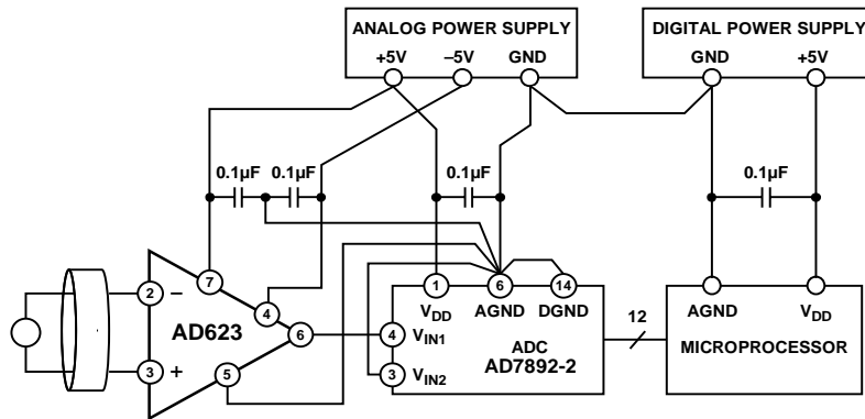
Figure 76. Optimal Grounding Practice for a Bipolar Supply Environment with Separate Analog and Digital Supplies
