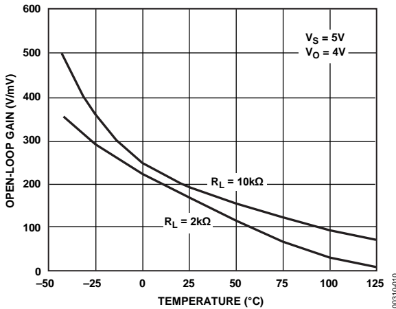
Figure 10. OP292 Open-Loop Gain vs. Temperature @ 5 V
