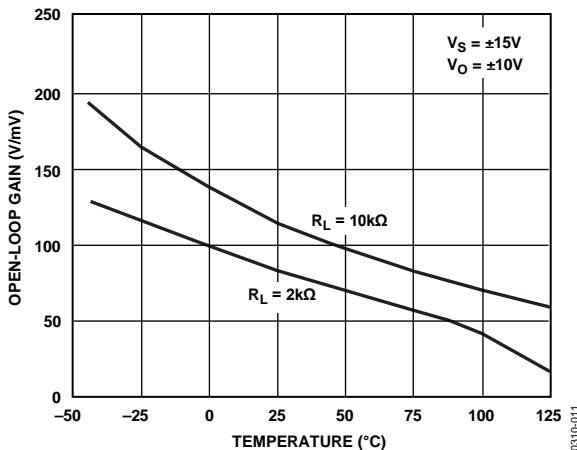
Figure 11. OP292 Open-Loop Gain vs. Temperature @ ±15 V
