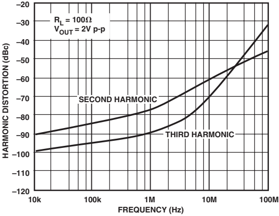
TPC 31. AD8048 Harmonic Distortion vs. Frequency, G = +2
