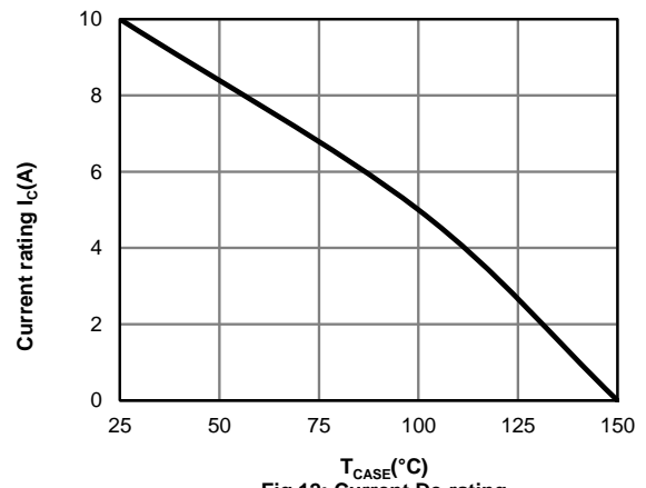
Fig 12: Current De-rating
