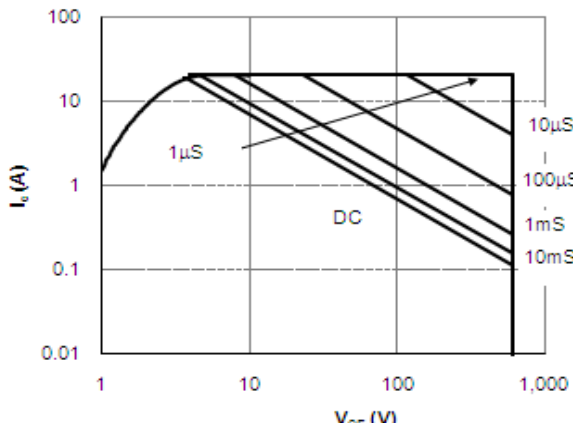
Fig 9: Forward Bias Safe Operating Area ( T_c=25^\circ\text{C}, V_{GE}=15\text{V} )
