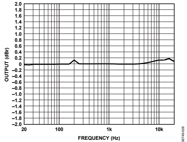
Figure 26. Frequency Response @ 1 W, 6 Ω, PVDD = 15 V, PGA = 0 dB
