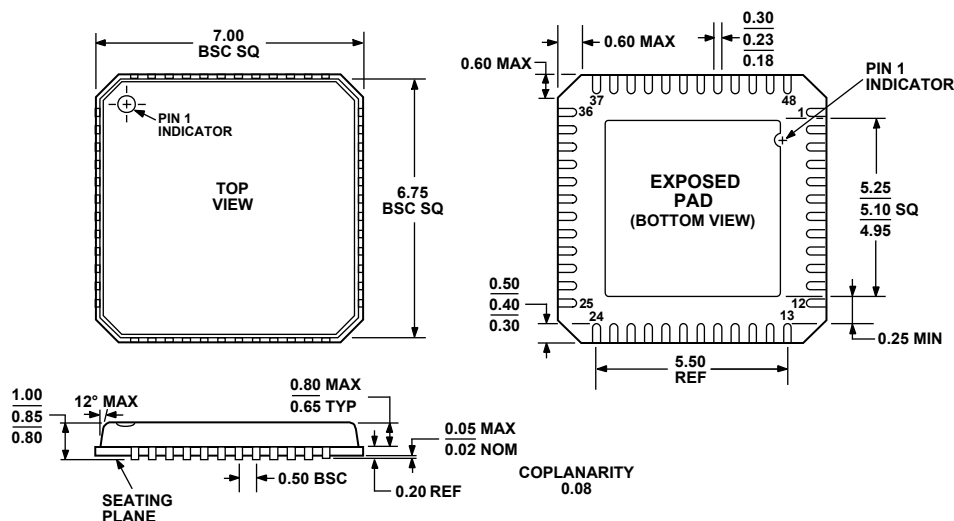
Figure 51. 48-Lead Lead Frame Chip Scale Package [LFCSP_VQ] 7 mm × 7 mm Body, Very Thin Quad (CP-48-1) Dimensions shown in millimeters
