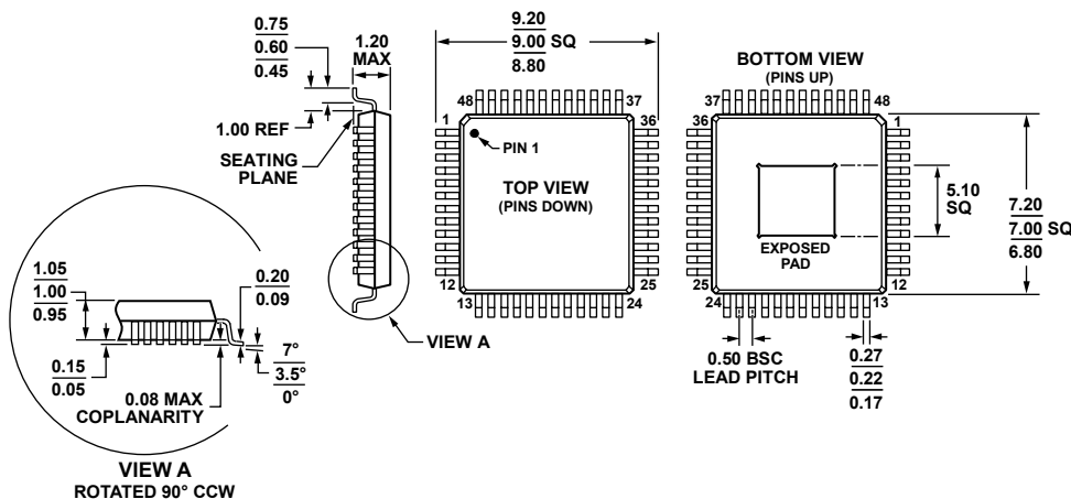
Figure 52. 48-Lead Thin Quad Flat Package, Exposed Pad [TQFP_EP] (SV-48-5) Dimensions shown in millimeters
