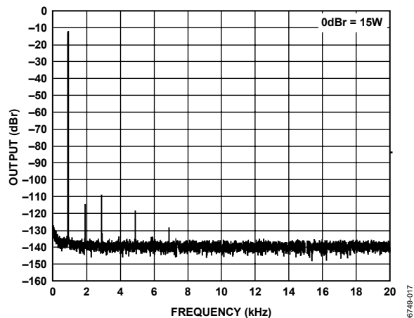
Figure 17. FFT @ 1 W, 6 Ω, PVDD = 15 V, PGA = 0 dB, 1 kHz Sine
