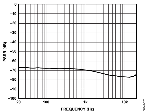
Figure 28. PSRR vs. Frequency, No Input Signal, Ripple = 1.5 V p-p, PVDD = 15 V, 6 Ω
