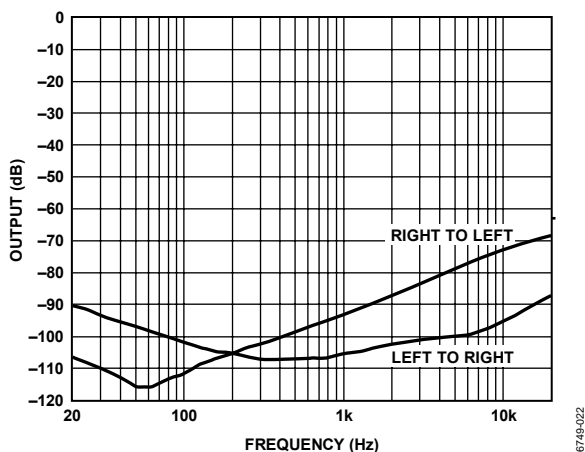
Figure 22. Crosstalk @ Full Scale, 6 Ω, PVDD = 15 V, PGA = 0 dB
