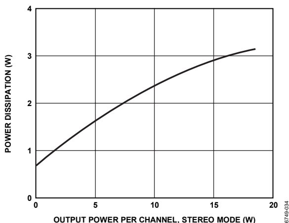
Figure 34. Power Dissipation vs. Output Power, 15 V, 8 Ω, Stereo Mode, Both Channels Driven
