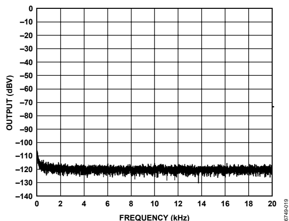
Figure 19. FFT No Input, 6 Ω, PVDD = 15 V, PGA = 0 dB
