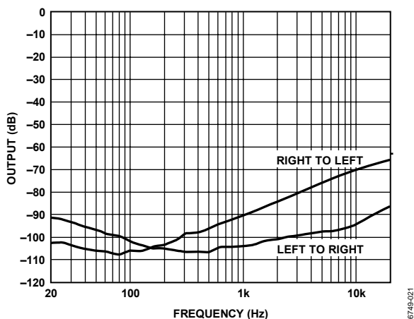
Figure 21. Crosstalk @ 1 W, 6 Ω, PVDD = 15 V, PGA = 0 dB
