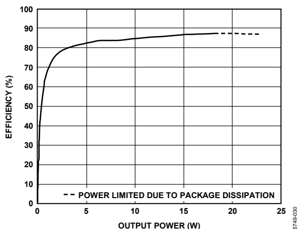
Figure 30. Efficiency vs. Output Power, 15 V, 6 Ω
