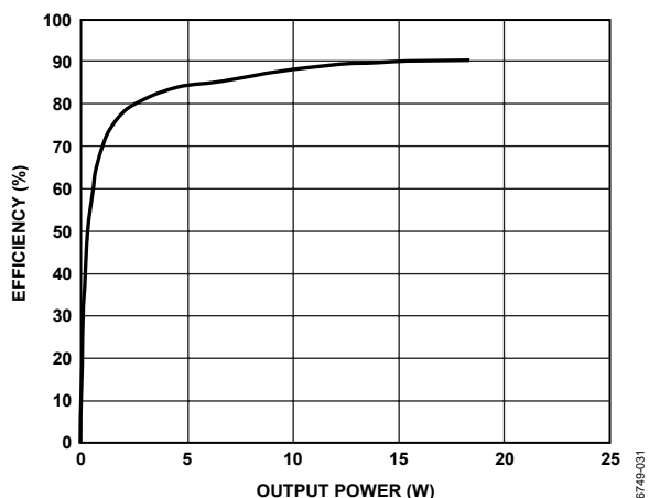
Figure 31. Efficiency vs. Output Power, 15 V, 8 Ω
