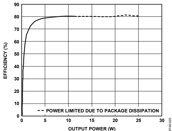
Figure 29. Efficiency vs. Output Power, 15 V, 4 Ω
