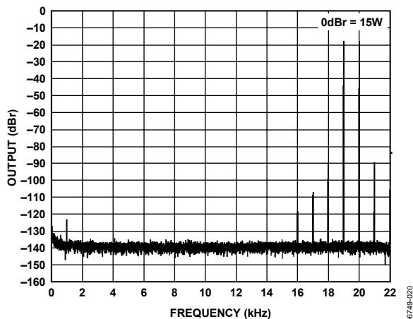
Figure 20. FFT @ 1 W, 6 Ω, PVDD = 15 V, PGA = 0 dB, 19 kHz and 20 kHz Sine
