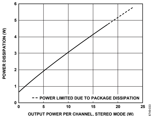
Figure 33. Power Dissipation vs. Output Power, 15 V, 6 Ω, Stereo Mode, Both Channels Driven
