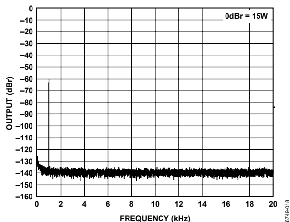
Figure 18. FFT @ -60 dBFS, 6 Ω, PVDD = 15 V, PGA = 0 dB, 1 kHz Sine
