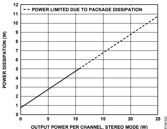
Figure 32. Power Dissipation vs. Output Power, 15 V, 4 Ω, Stereo Mode, Both Channels Driven
