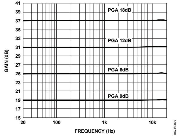
Figure 27. Gain vs. Frequency @ 1 W, 6 Ω, PVDD = 15 V
