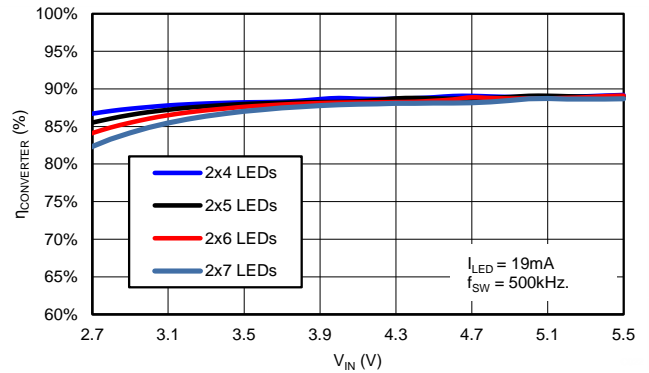
Figure 24. Backlight Efficiency vs Input Voltage Dual String
