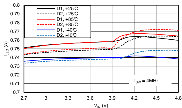
Figure 4. Flash LED Current Line Regulation @ f_{SW} = 4\text{MHz}
