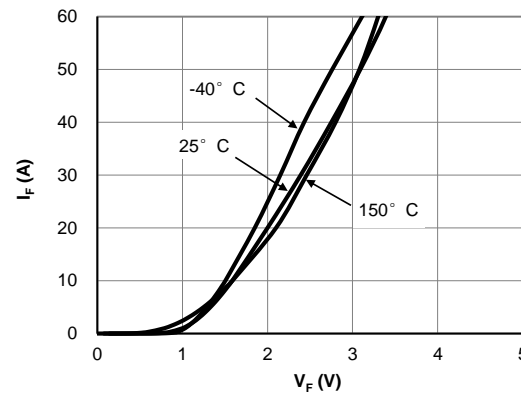
Figure 4: Diode Characteristic
