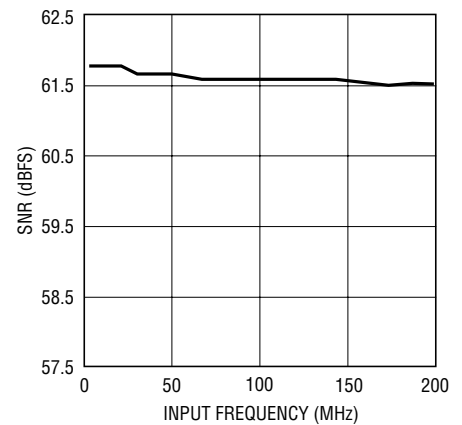
LTC2236: SNR vs Input Frequency, -1\text{dB} , 2\text{V} Range, 25\text{Msps}
