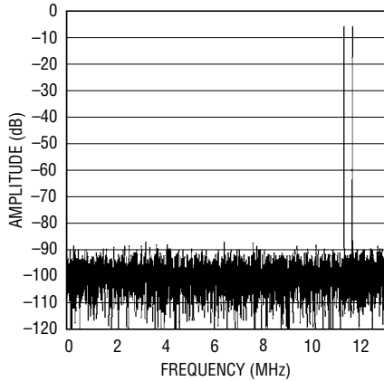
LTC2236: 8192 Point 2-Tone FFT, f_{IN} = 10.9\text{MHz} and 13.8\text{MHz} , -1\text{dB} , 2\text{V} Range, 25\text{Msps}
