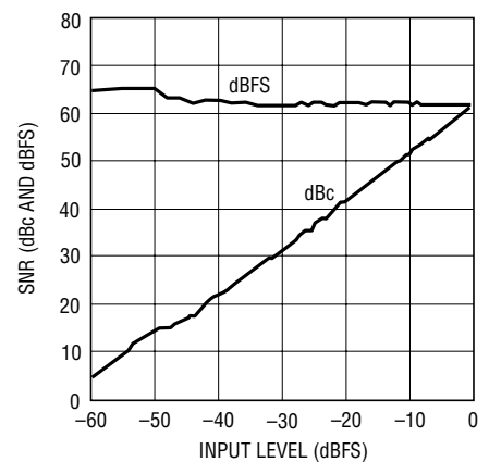
LTC2236: SNR vs Input Level, f_{IN} = 5\text{MHz} , 2\text{V} Range, 25\text{Msps}
