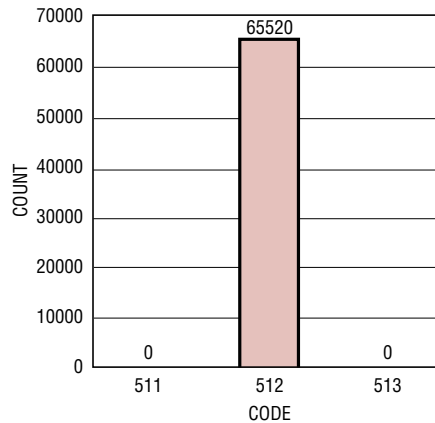
LTC2236: Grounded Input Histogram, 25\text{Msps}
