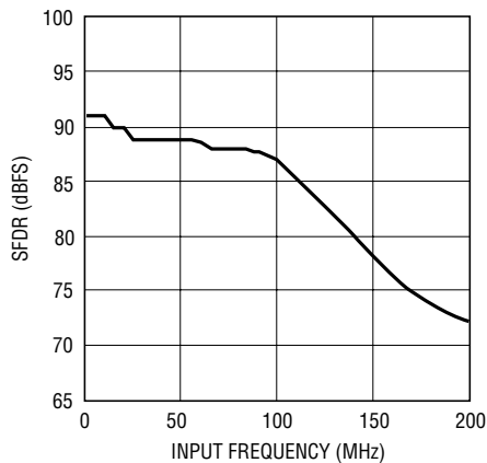
LTC2236: SFDR vs Input Frequency, -1\text{dB} , 2\text{V} Range, 25\text{Msps}
